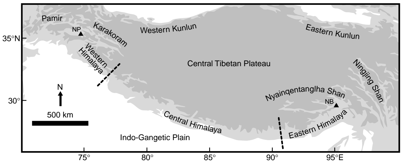
Figure 1. Generalized topographic map of the Himalaya and Tibetan Plateau. Dark shading indicates elevations above 4000 m; light shading indicates elevations between 1000 and 3000 m. Dashed lines represent boundaries between the western, central, and eastern Himalaya. NP—Nanga Parbat; NB—Namche Barwa.
